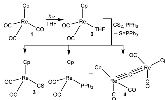
Scheme 2. Synthesis of a dirhenium \mu -carbido complex ( 4 ; \text{Cp} = \eta\text{-C}_5\text{H}_5 ).
